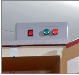
Control unit with fire detection Malfunction message via optical signal and switch-off of the ventilation system.
