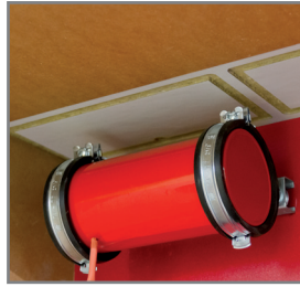
Fire suppression system Current-independent tripping in the event of fire and impermissible temperature rise.
